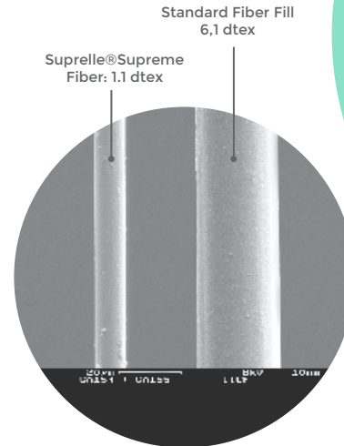
Picture taken with an electronic microscope SEM (Scanning Electron Microscope) enlarged 1,000 times.
